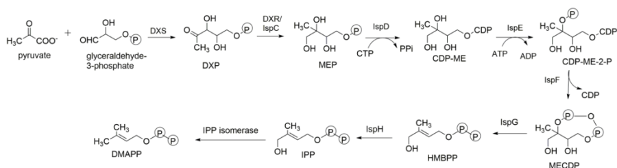
Fig. 5.4 Biosynthesis of Decaprene.
