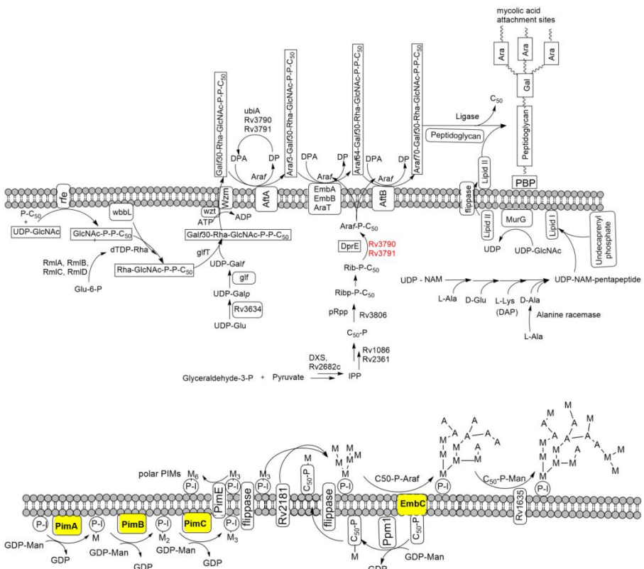
Fig. 5.3 Mycolyl-Arabinogalactan-Peptidoglycan Complex. 19-21
